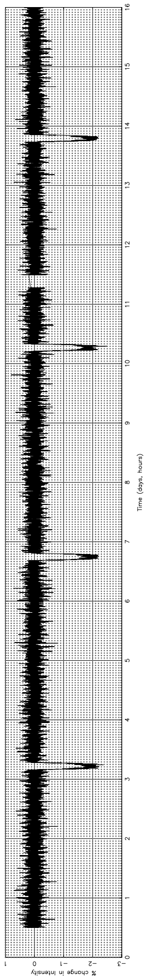
MOST Observations HD 209458
